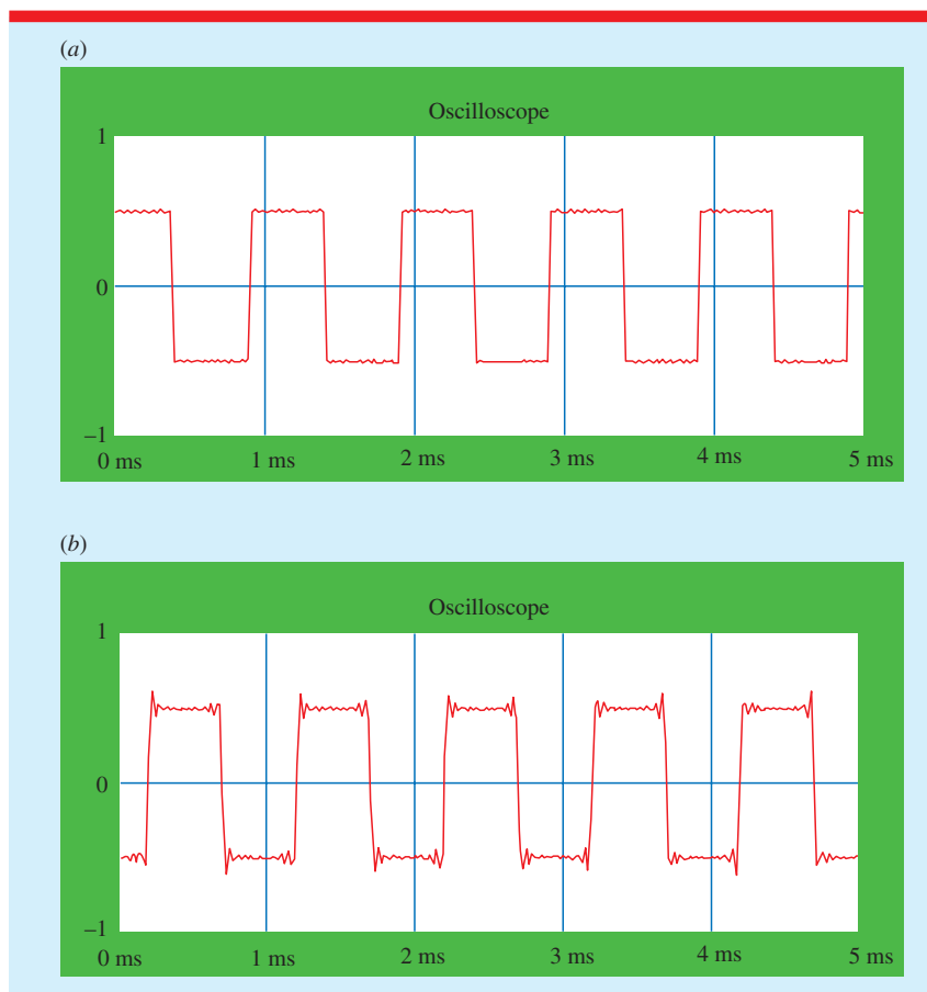
Figure 3. (a) A 1000 Hz square wave on the Mac with Google Chrome. Note that this rendition is better than what is displayed on the PC seen in figure (b). (b) A 1000 Hz square wave on a PC with Google Chrome. Note that this PC has trouble with the higher-frequency components of the square wave, essentially filtering out higher harmonics. The Mac (figure (a)) does a better job reproducing the square wave.
