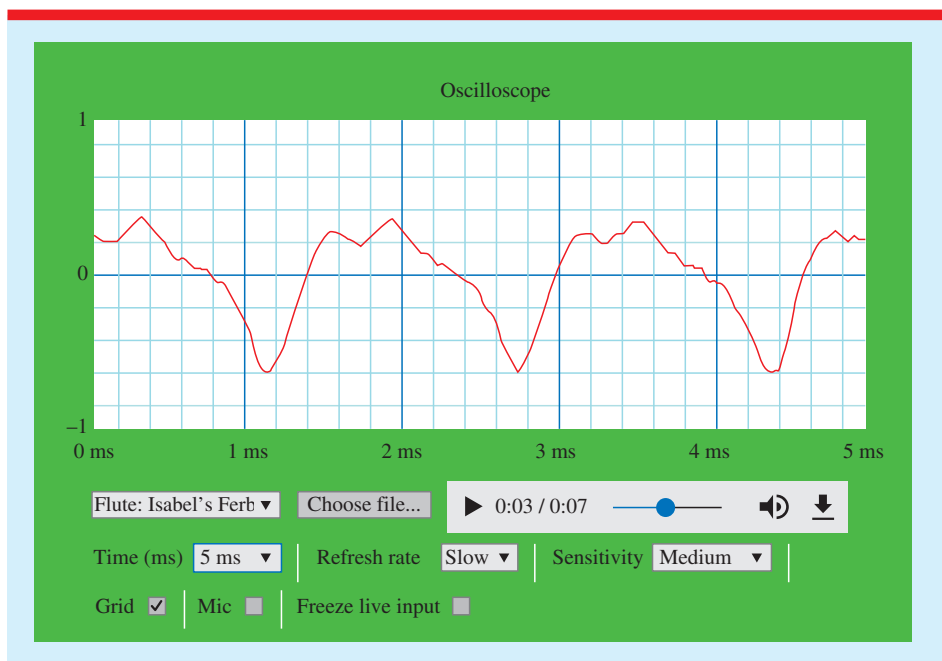
Figure 1. Screenshot of waveform produced by a flute, courtesy flautist Isabel Ferber.
