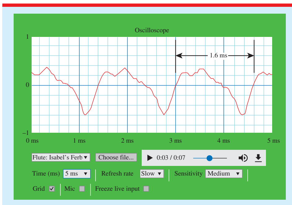
Figure 2. Measuring the period of a periodic wave on the oscilloscope.
